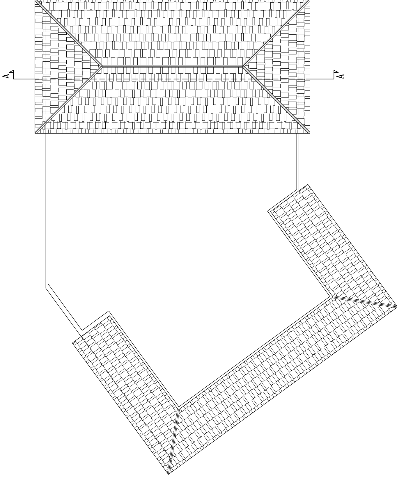
ROOF PLAN BLOCK F
